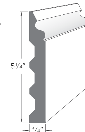
Colonial Base Cap AZM-163
