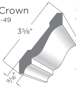
Rams Crown AZM-6934
