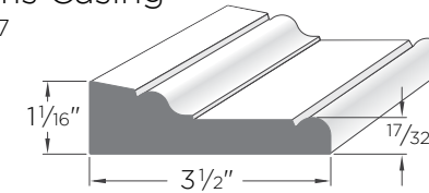
Back Band AZM-6931
