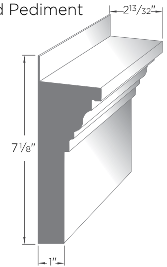
Fluted / Reeded AZM-606
