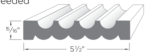
Garage Door Thermostop AZM-6936
